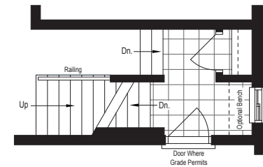
MAIN FLOOR LAYOUT WITH SECOND FLOOR LAUNDRY
