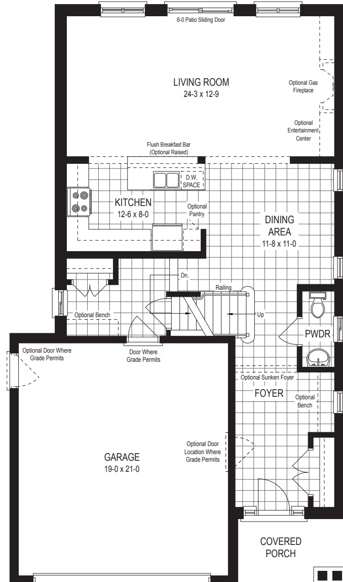
MAIN FLOOR
