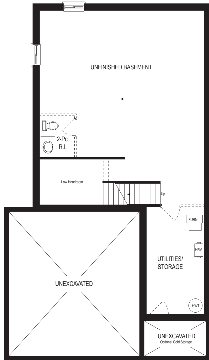
BASEMENT FLOOR
